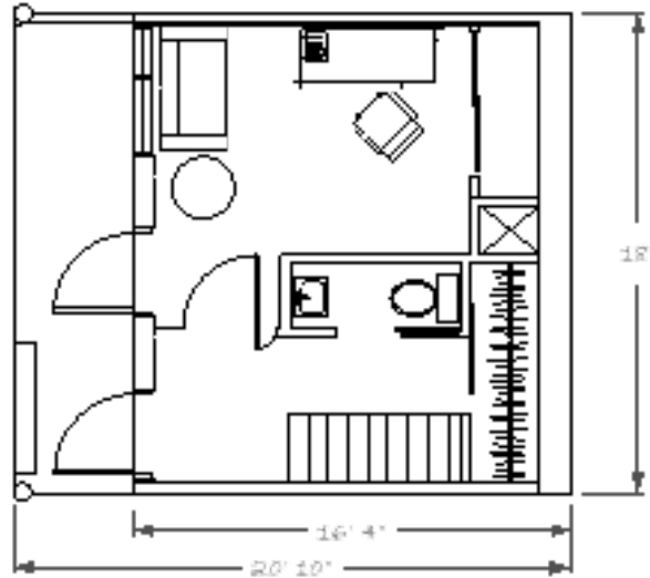
MEZZANINE (TOÎT) / (ROOF)
